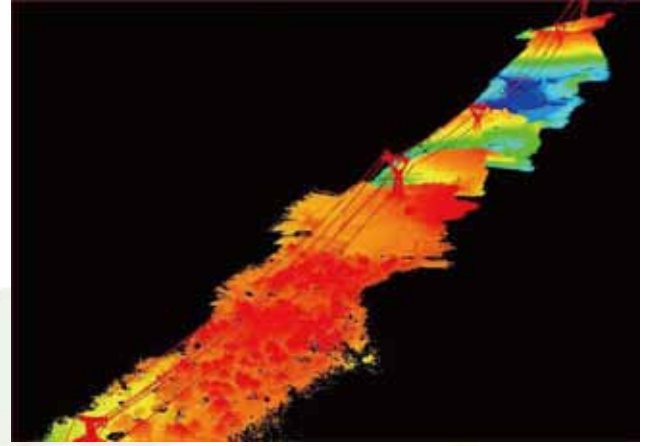
Powerline laser point cloud
